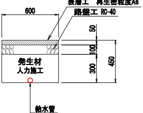
宅内As
